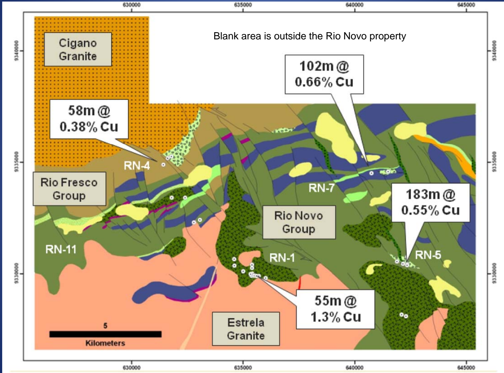
Figure 2: Southern Portion of Rio Novo Geology & Selected Intersections
